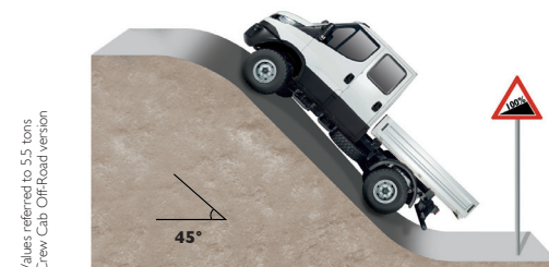
Maximum grade-ability
